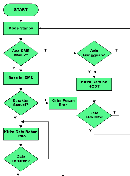
GAMBAR 7. Flowchart Alur Program Remote Unit.
